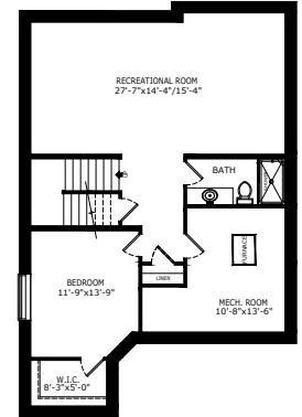
1 BEDROOM 'LEGAL SUITE' 848 SQ FT
