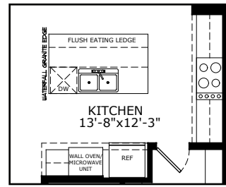
OPTIONAL EXECUTIVE KITCHEN
