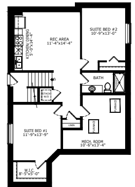
2 BEDROOM 'LEGAL SUITE' 848 SQ FT
